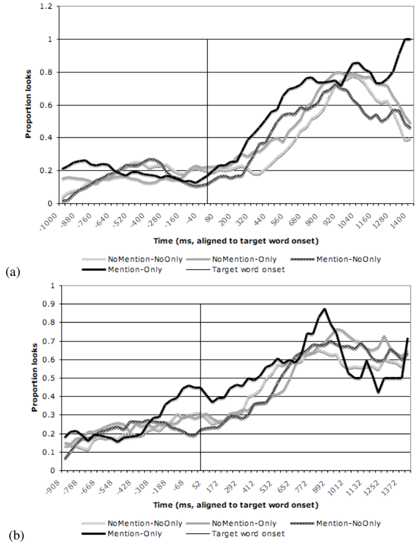
Figure 5: Experiment 2. Proportion looks to the target item in (a) Underinformative context, (b) Informative context conditions. Aligned to target word onset.
