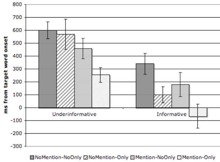
Figure 6: Experiment 2. Average time to target convergence.
