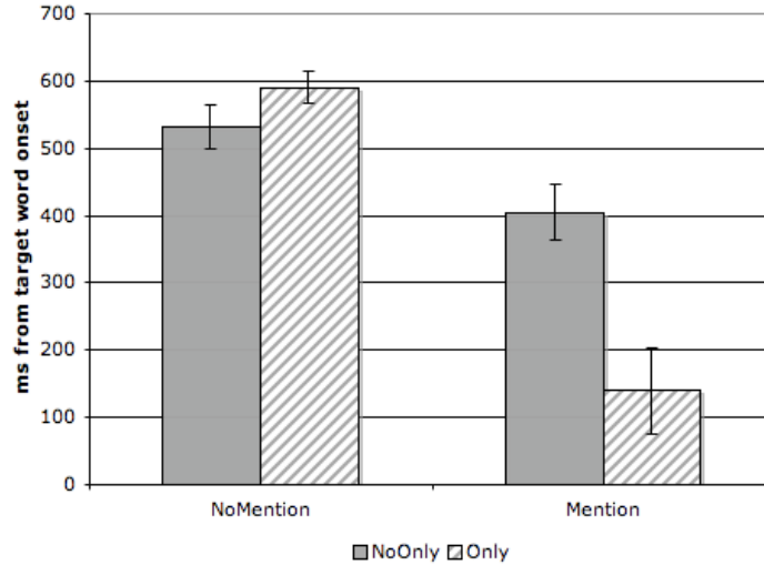
Figure 3: Experiment 1. Average time to target convergence.
